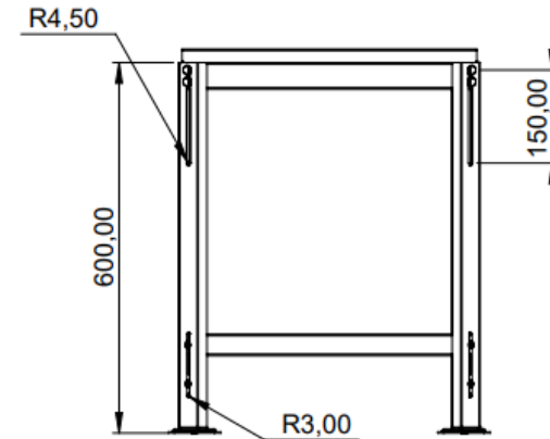
600mm Ground Base
