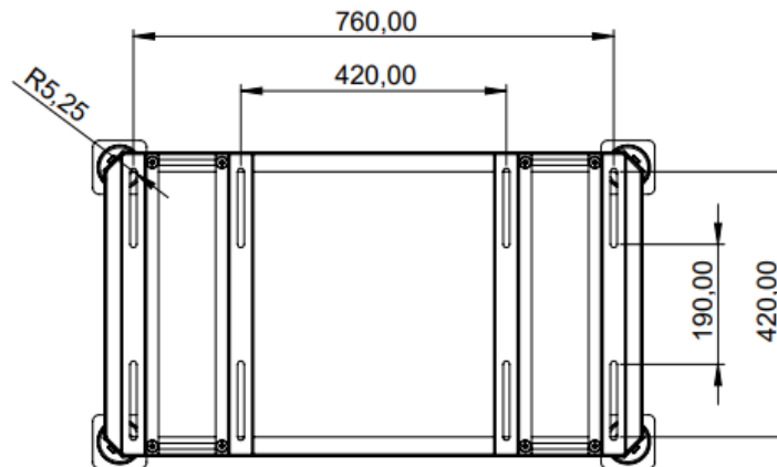
Detail view for connection
